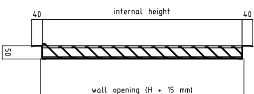
cross-section
